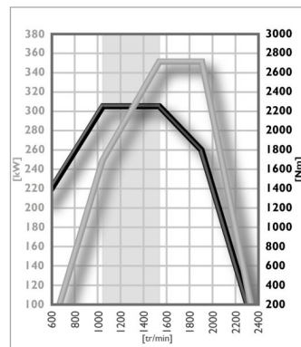
engine power - torque - RPM
